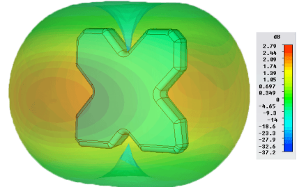
3D Gain Plot (950MHz)
